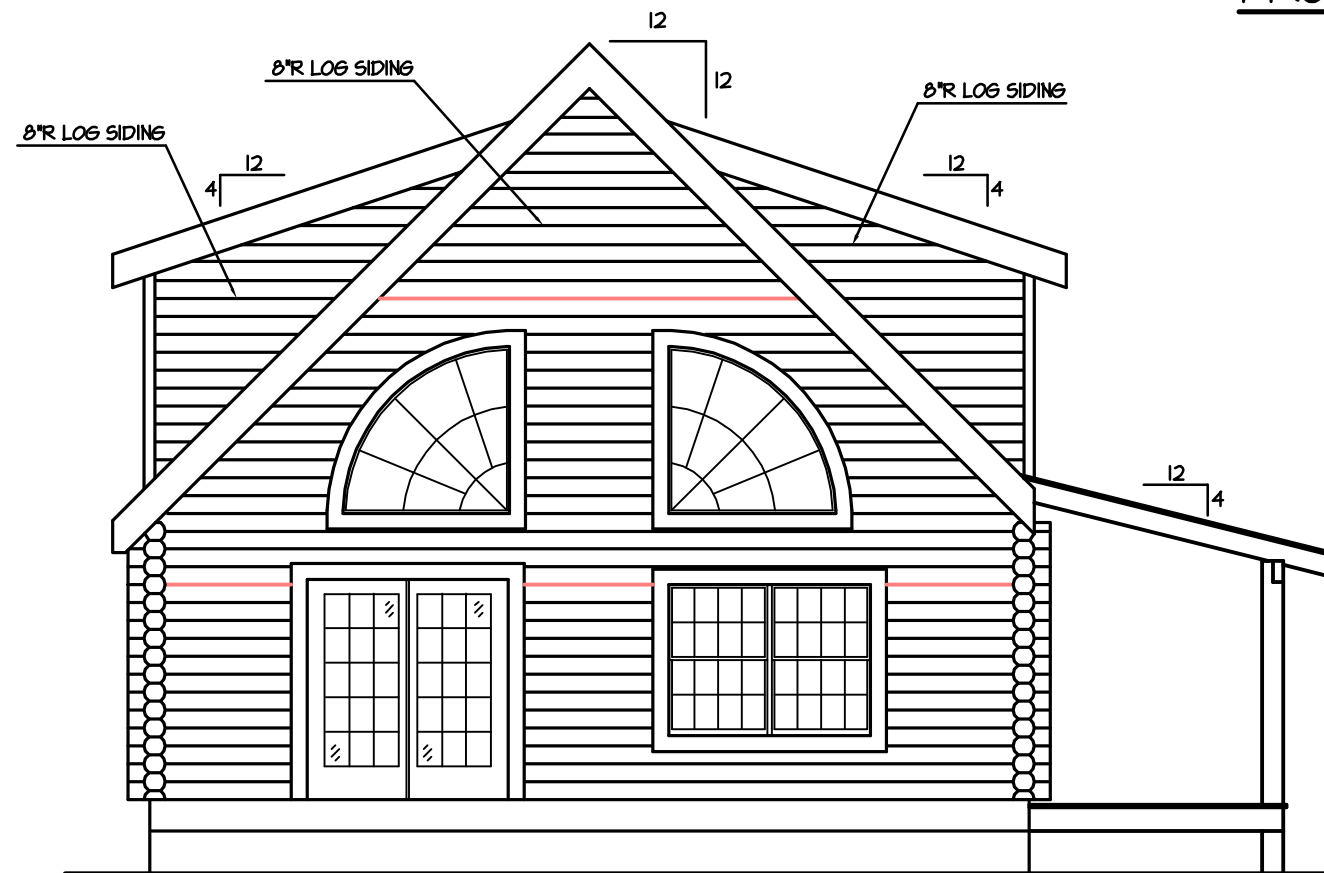
LEFT ELEVATION
