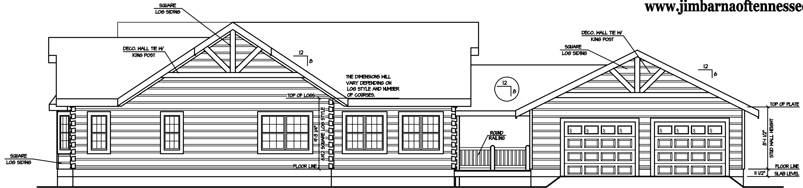
RIGHT ELEVATION 1/4" = 1'-0"
