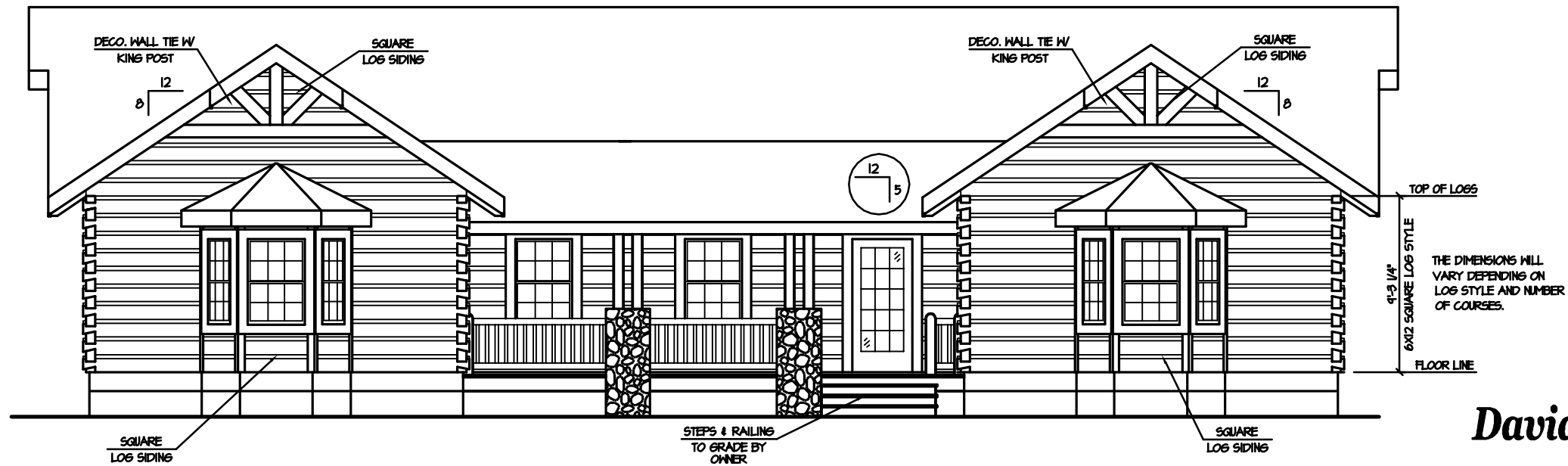
FRONT ELEVATION 1/4" = 1'-0"
