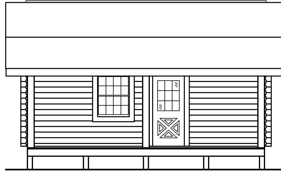
FRONT ELEVATION 1/4" = 1'-0"
