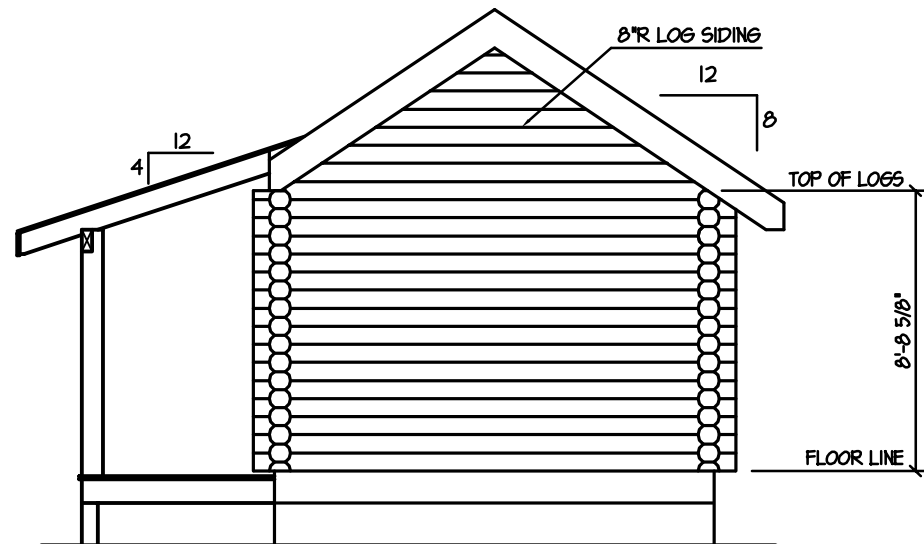
RIGHT ELEVATION 1/4" = 1'-0"
