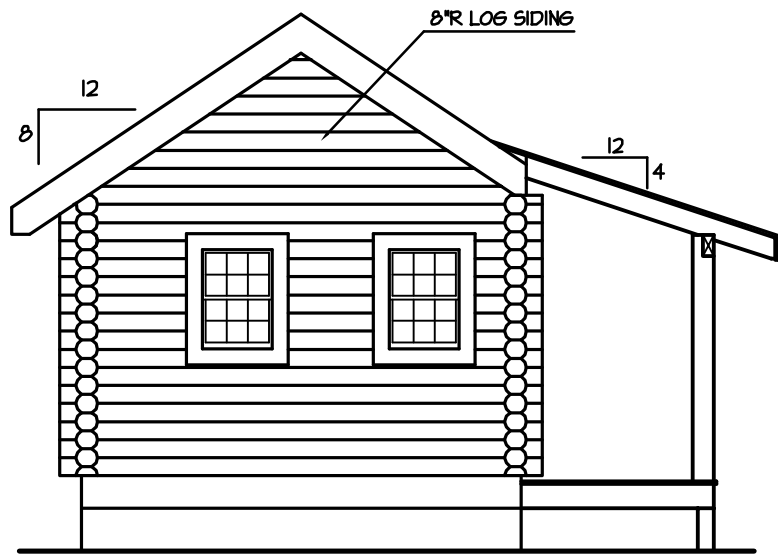
LEFT ELEVATION 1/4" = 1'-0"
