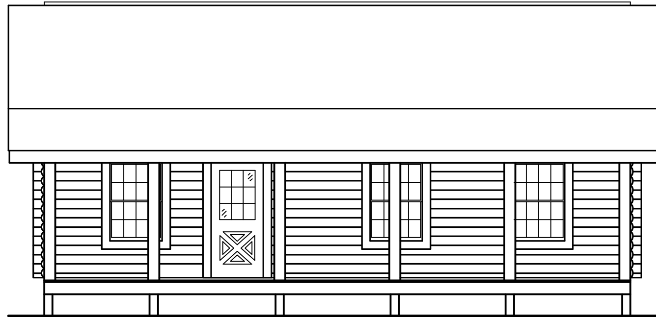
FRONT ELEVATION
