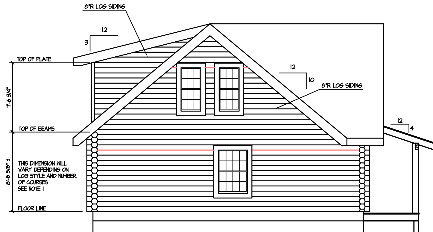
LEFT ELEVATION
