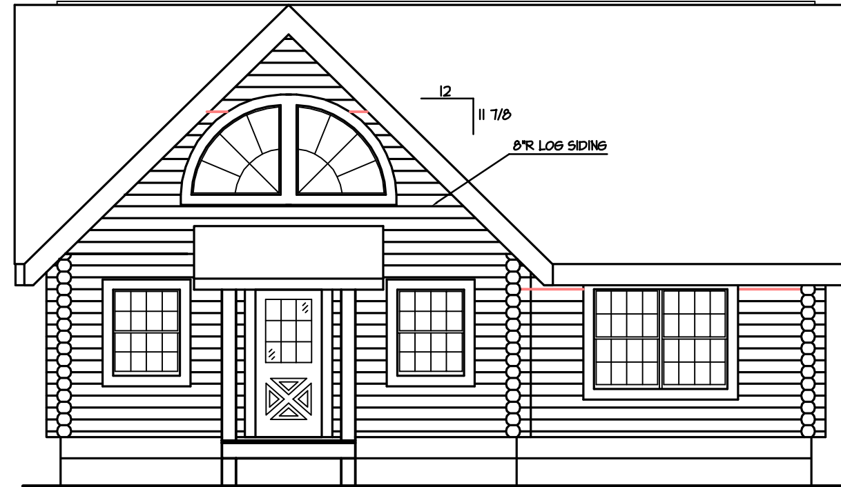
FRONT ELEVATION
