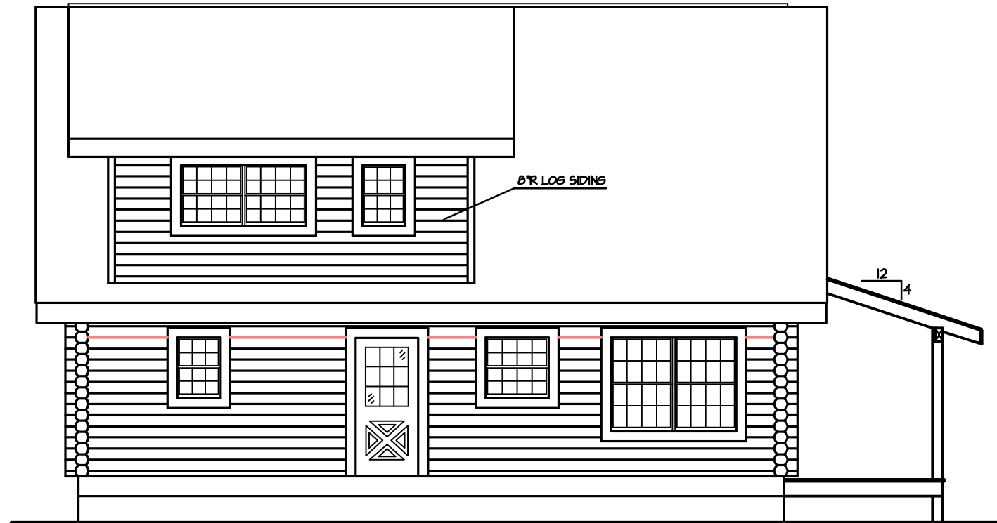
LEFT ELEVATION 1/4" = 1'-0"
