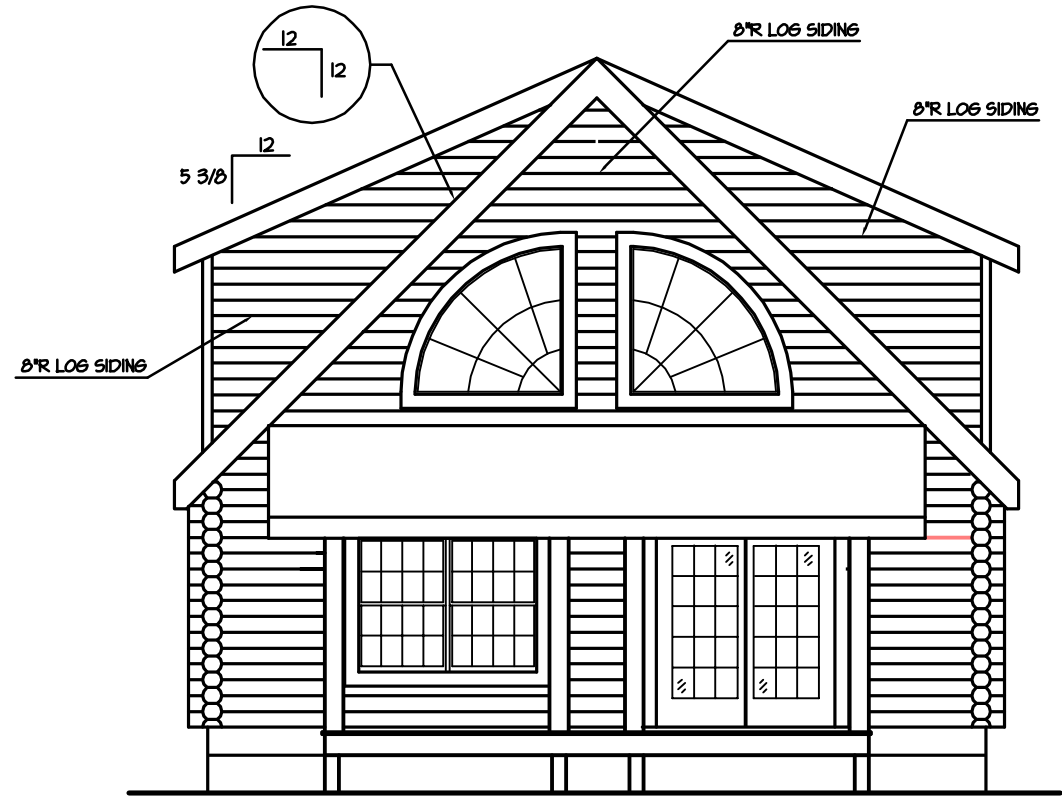
FRONT ELEVATION 1/4" = 1'-0"
