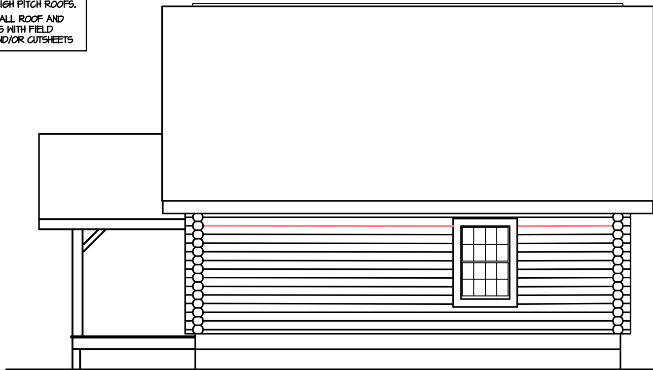
RIGHT ELEVATION 1/4" = 1'-0"
