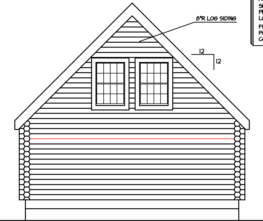
REAR ELEVATION 1/4" = 1'-0"
