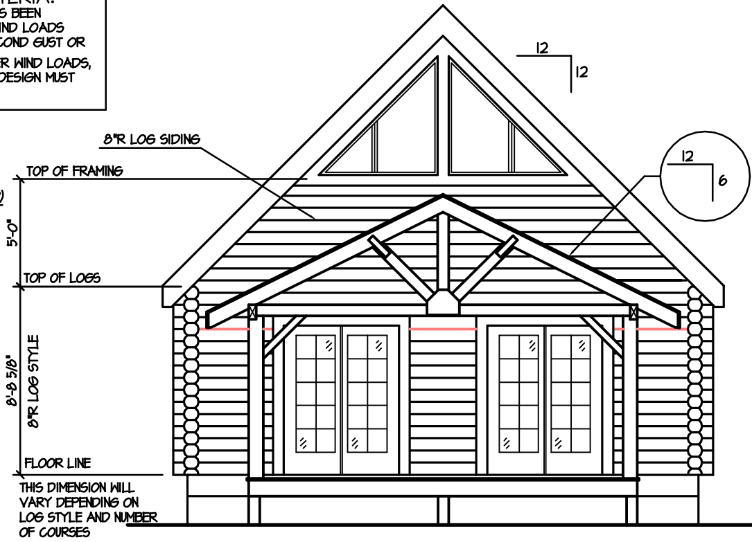
FRONT ELEVATION 1/4" = 1'-0"
