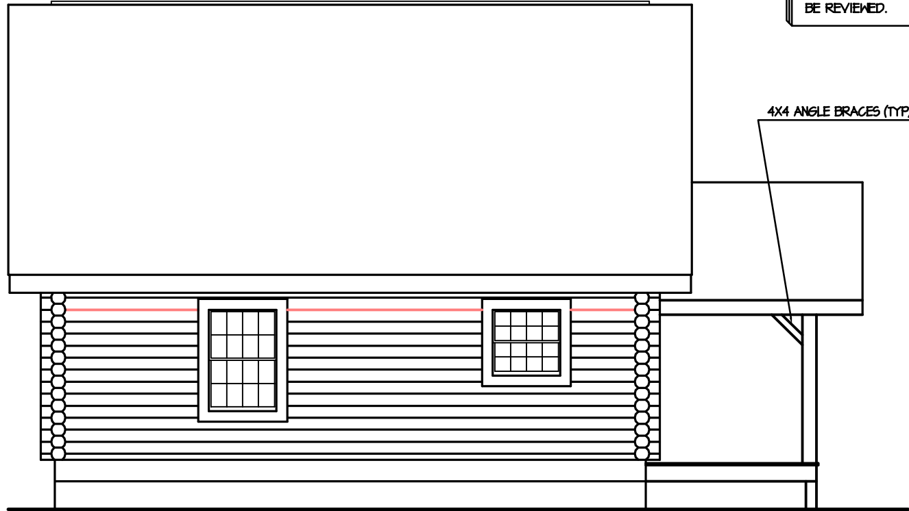
LEFT ELEVATION 1/4" = 1'-0"
