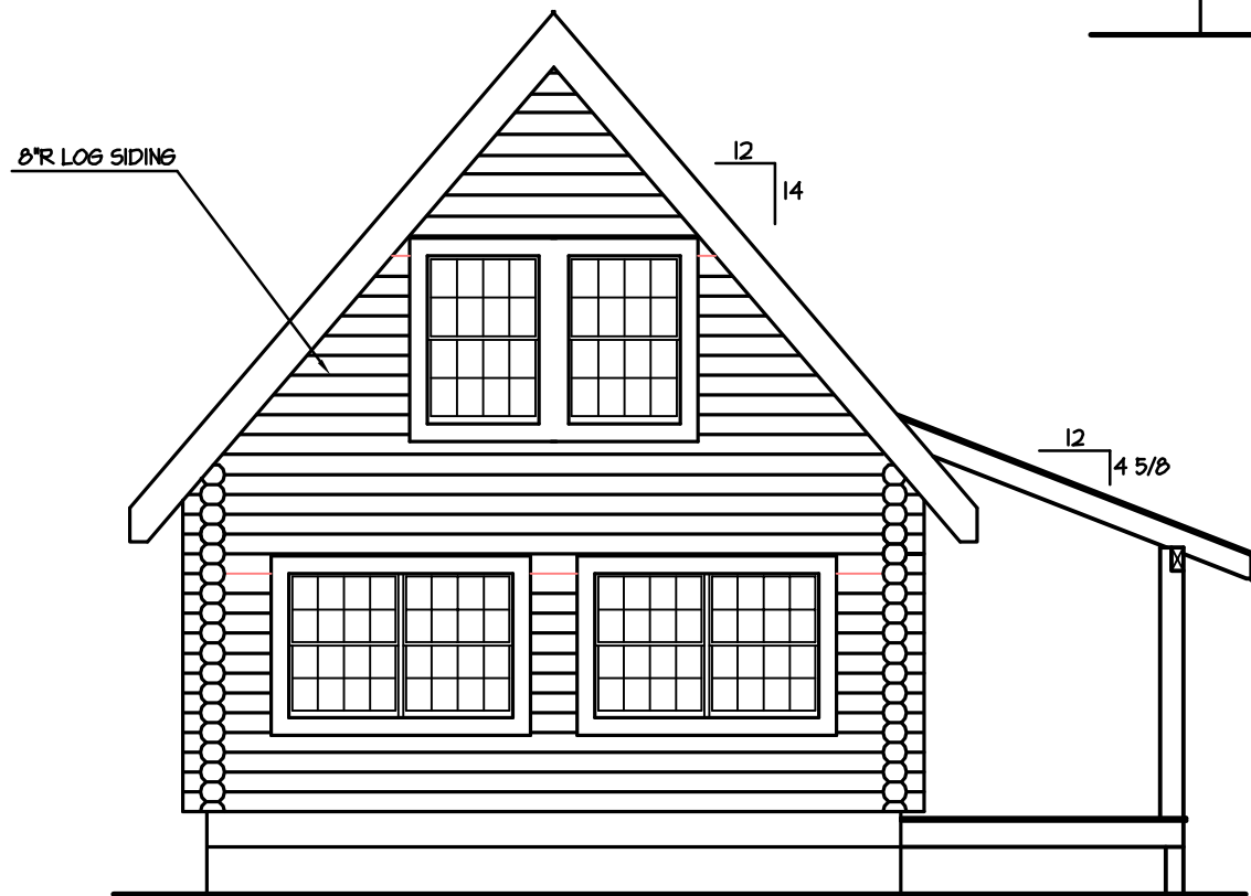
LEFT ELEVATION
