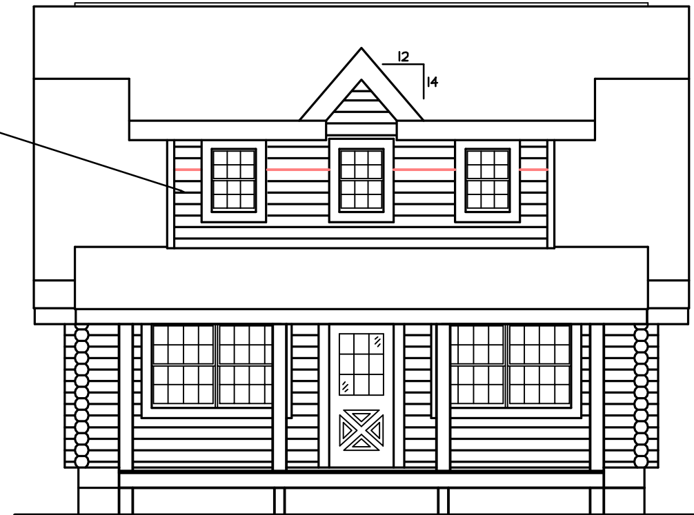
FRONT ELEVATION
