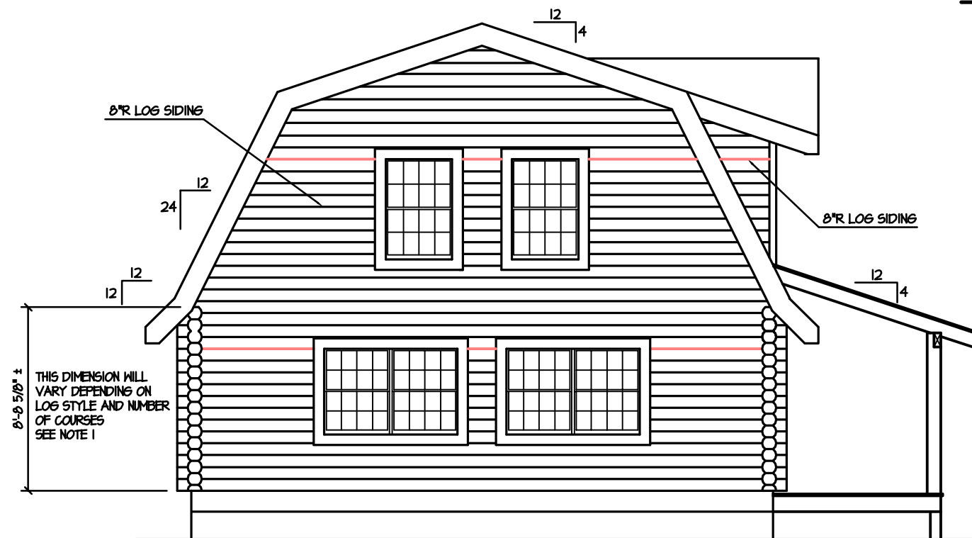
LEFT ELEVATION
