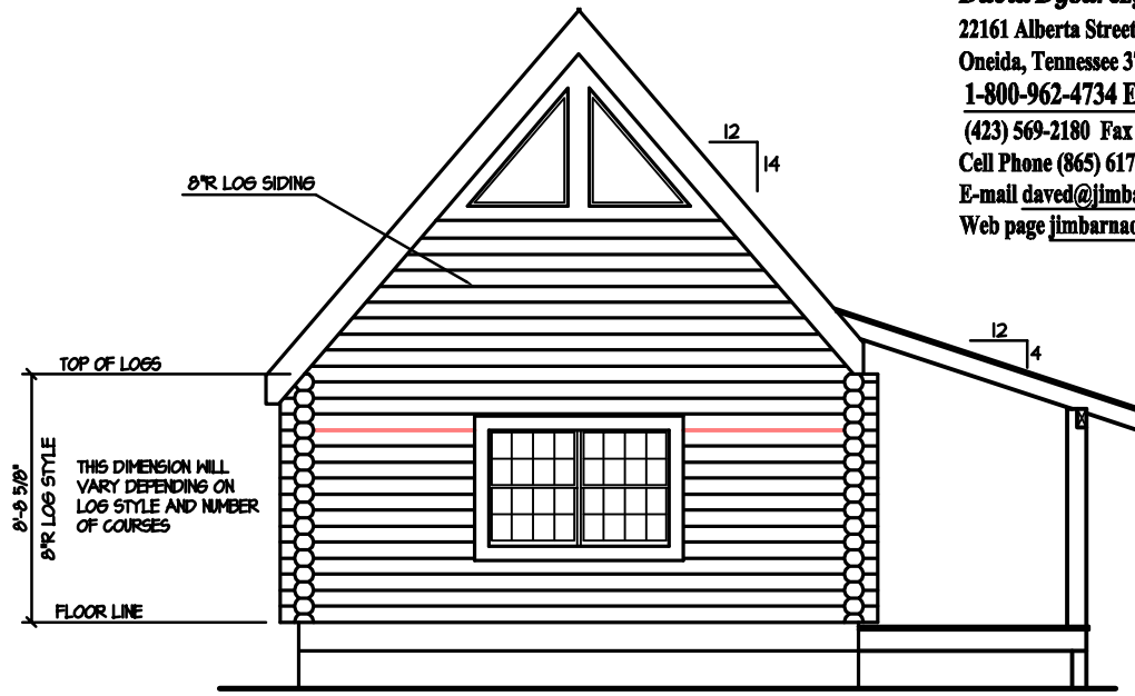
LEFT ELEVATION
