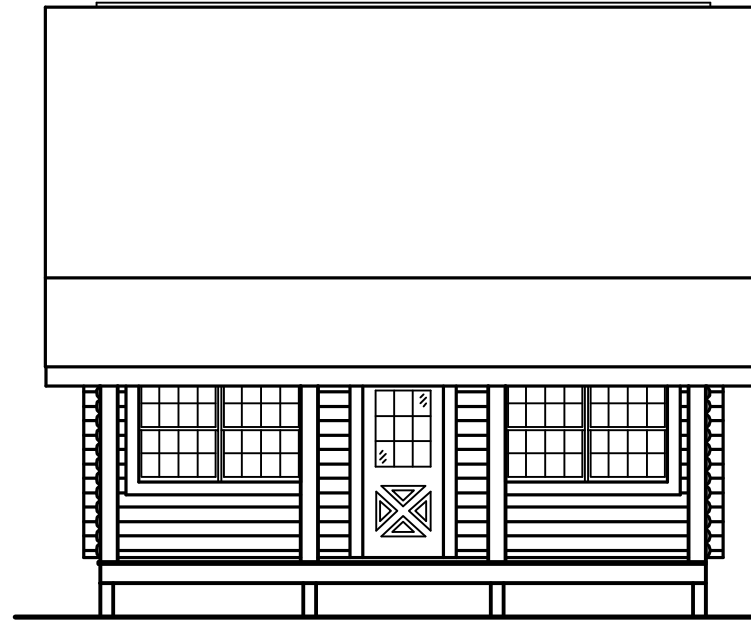
FRONT ELEVATION
