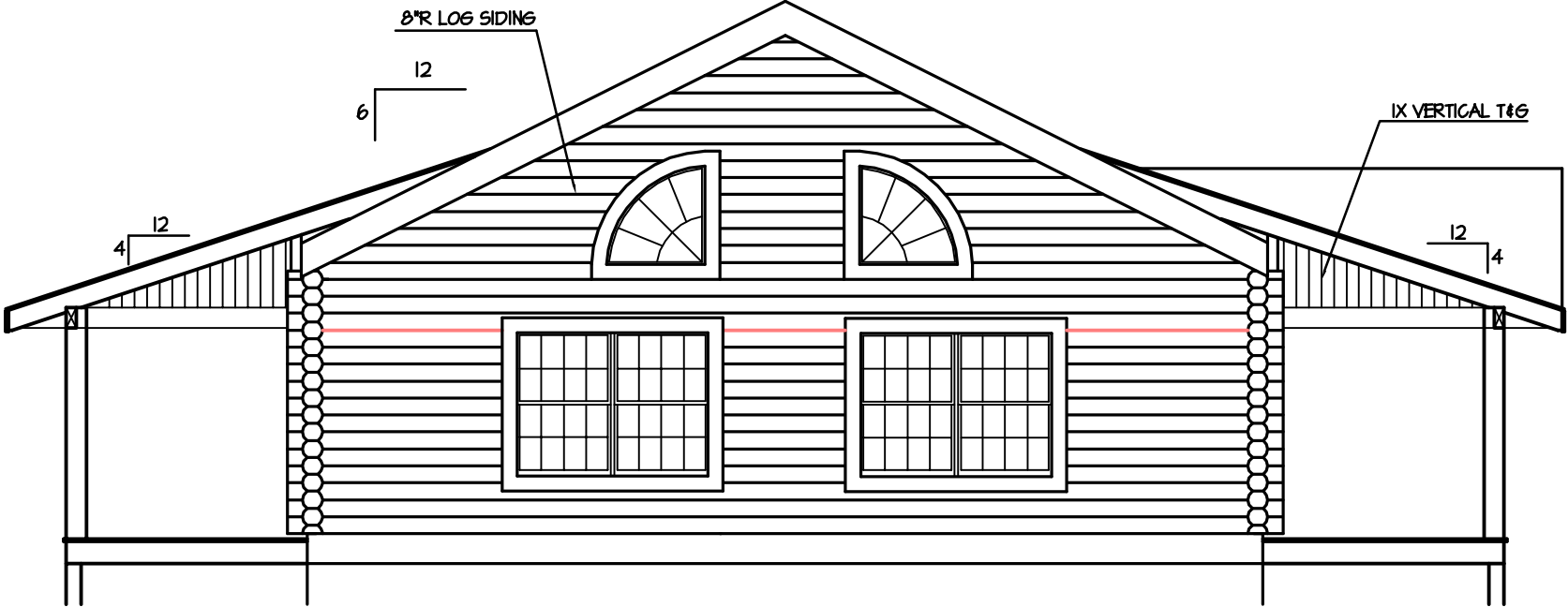
LEFT ELEVATION
