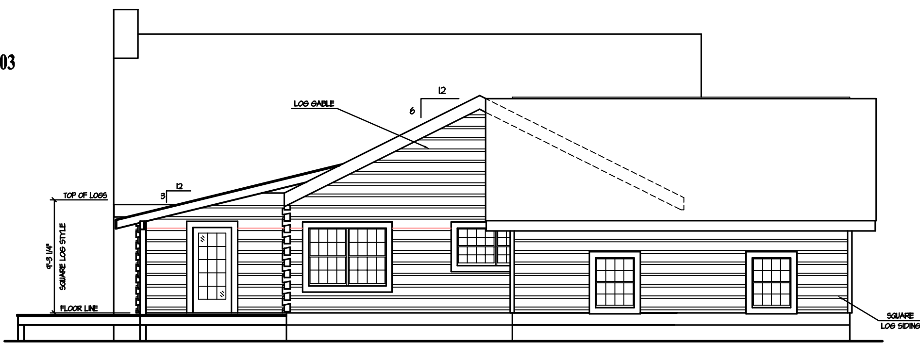
RIGHT ELEVATION 1/4" = 1'-0"
