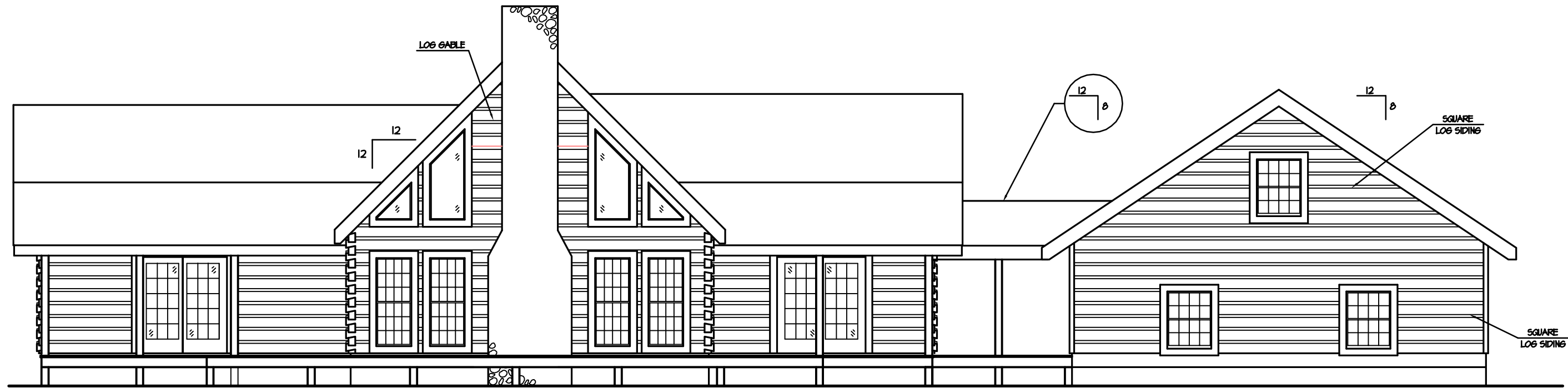
FRONT ELEVATION 1/4" = 1'-0"
