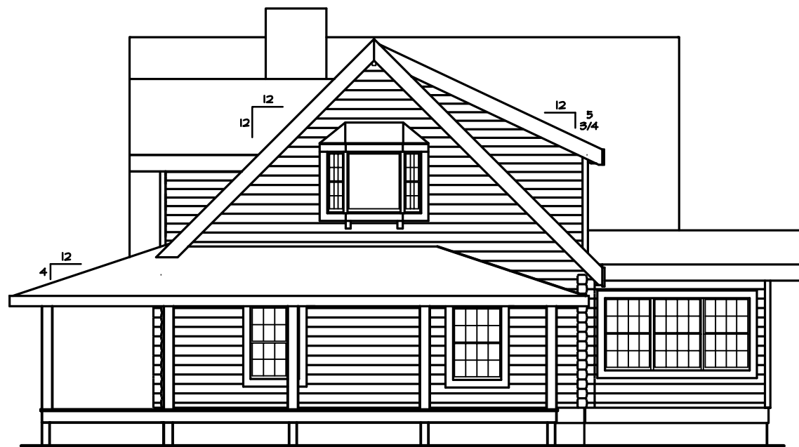
RIGHT ELEVATION 1/4" = 1'-0"
