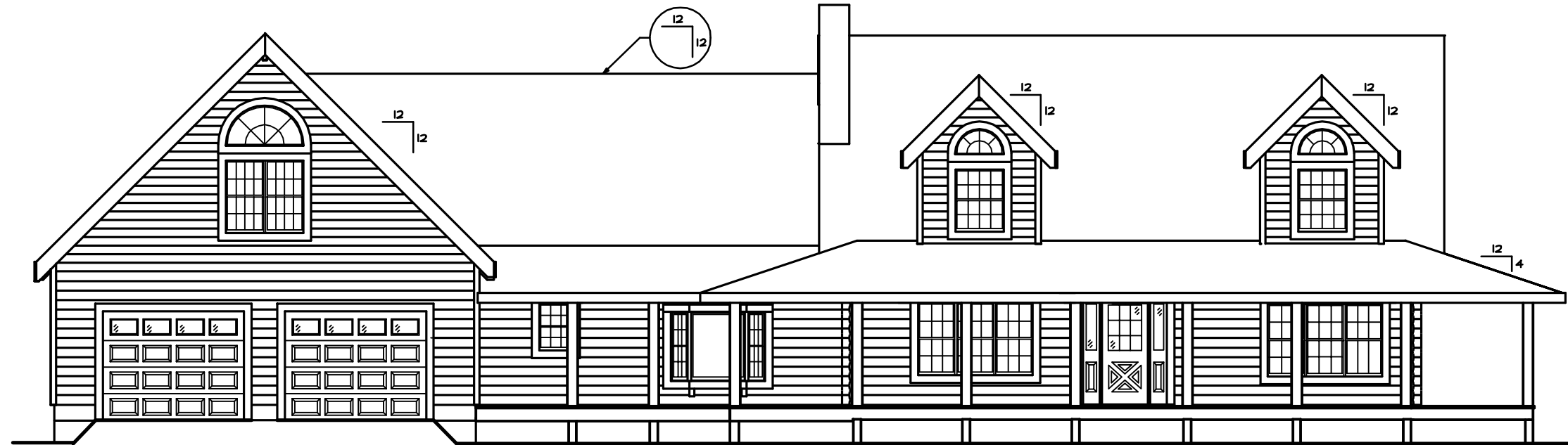
FRONT ELEVATION 1/4" = 1'-0"
