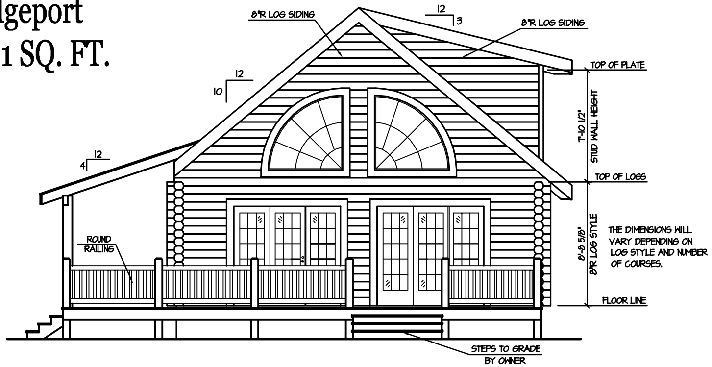
RIGHT ELEVATION 1/4" = 1'-0"
