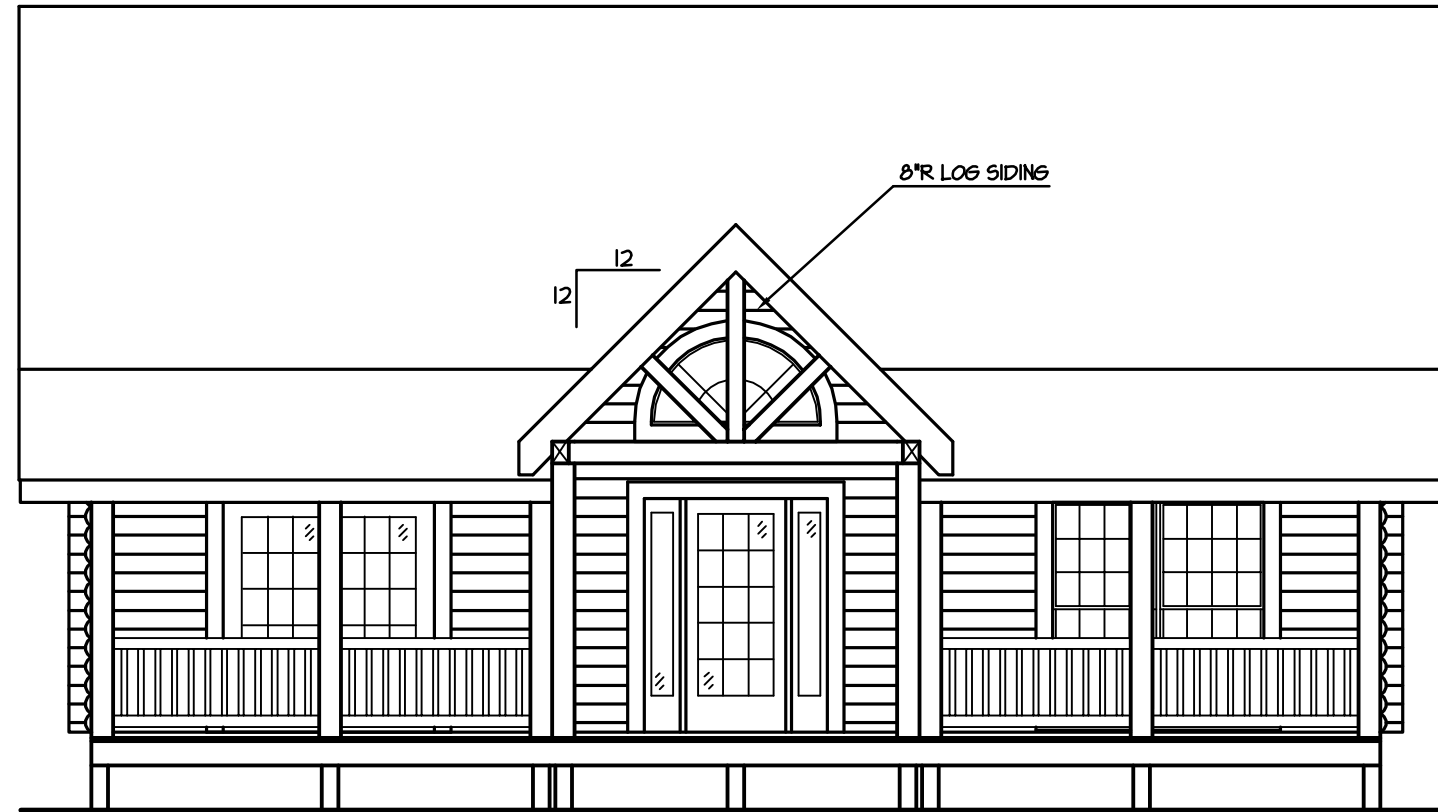
FRONT ELEVATION
