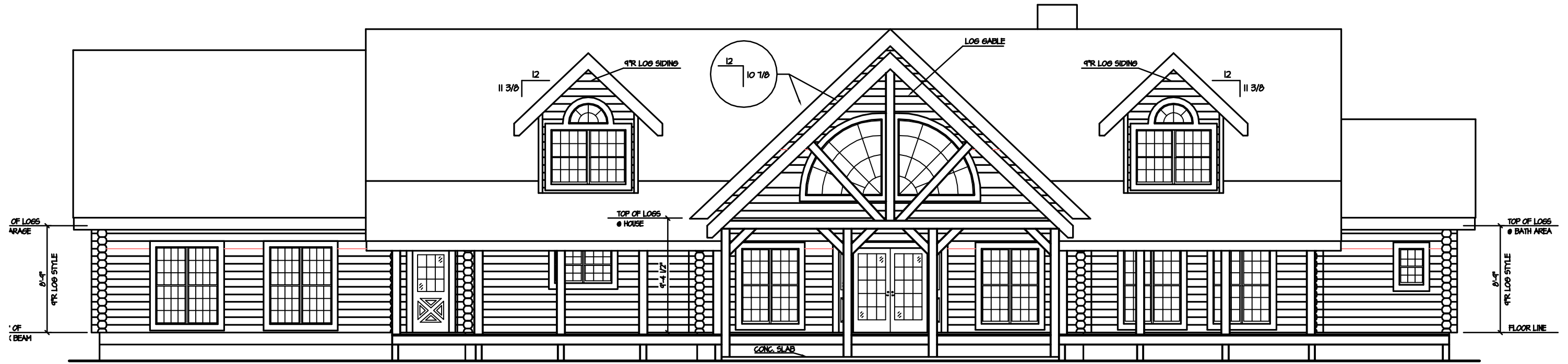
FRONT ELEVATION 1/4" = 1'-0"
