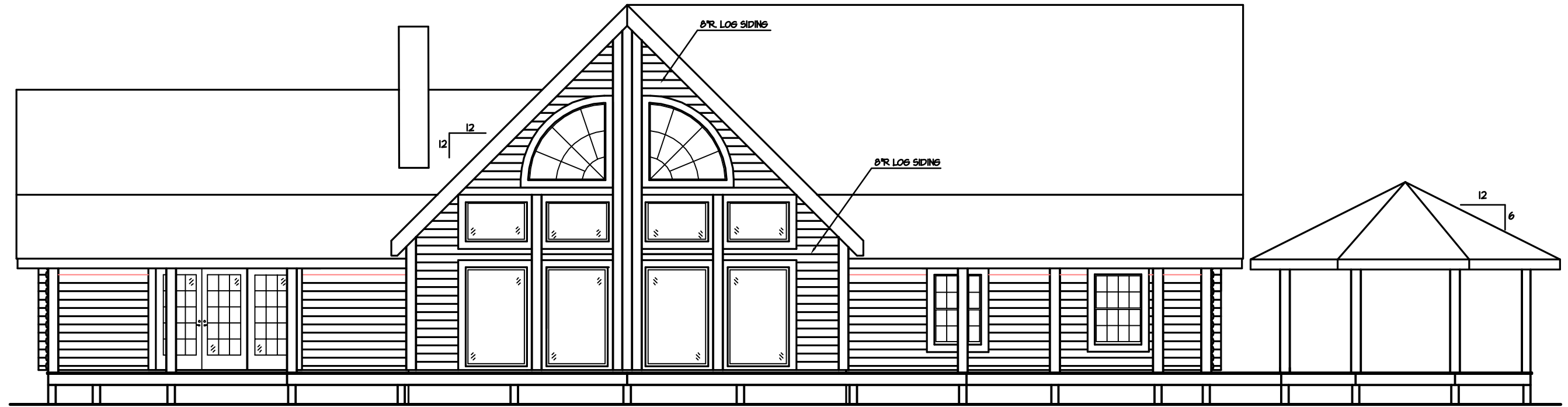
FRONT ELEVATION 1/4" = 1'-0"
