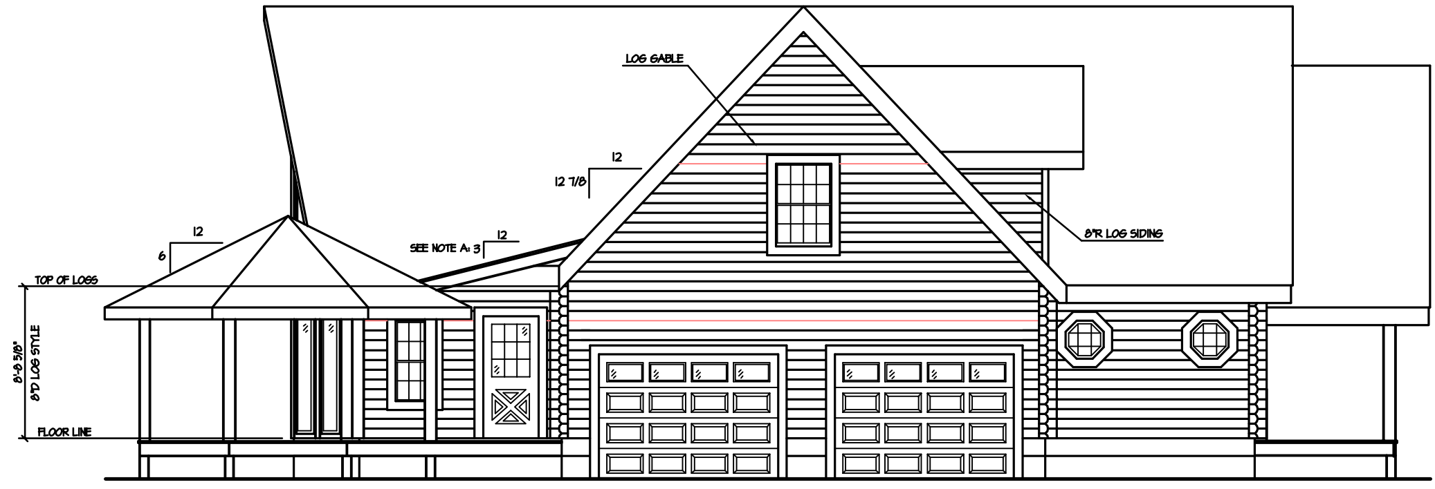
RIGHT ELEVATION 1/4" = 1'-0"
