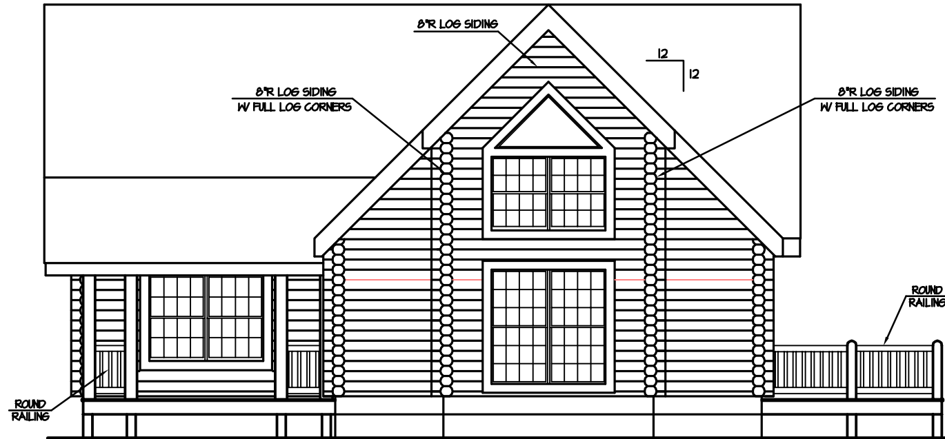
FRONT ELEVATION 1/4" = 1'-0"
